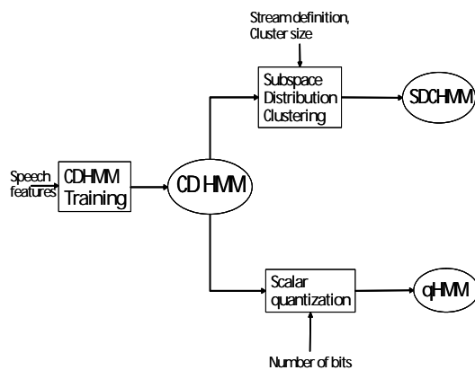
Figure 1. Derivation of qHMM and SDCHMM from CDHMM.
